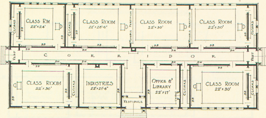
FLOOR PLAN No 6 SIX TEACHER COMMUNITY SCHOOL TO FACE EAST OR WEST ONLY
